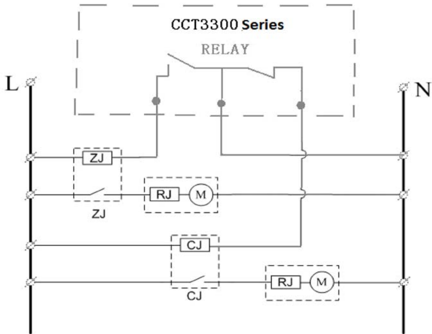
Connection diagram of ON/OFF relay
